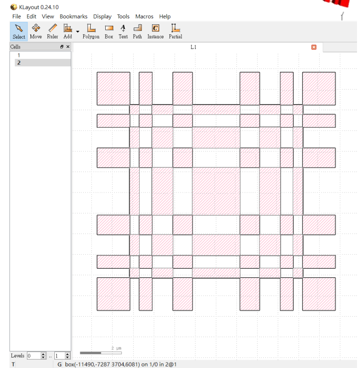
GDS-II Layout in KLayout
